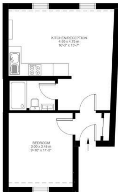
Third Floor
